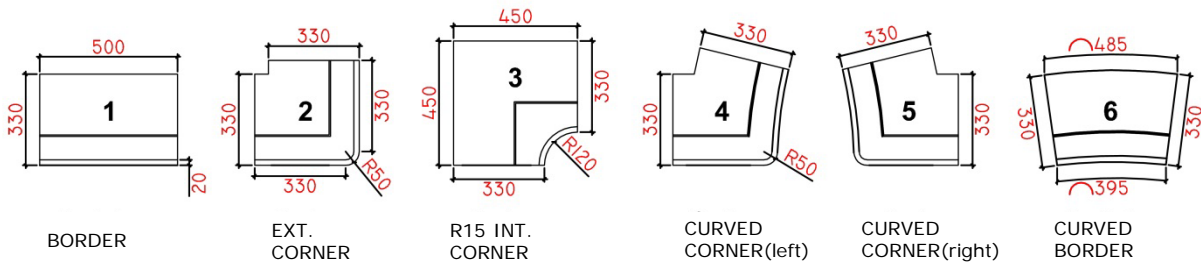
Assembly scheme
